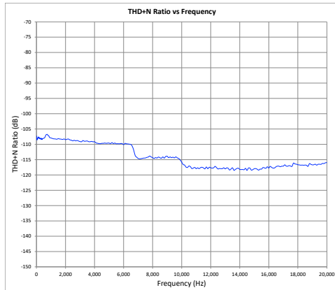
Figure 28: -1dBFS THD+N ratio Vs Frequency
