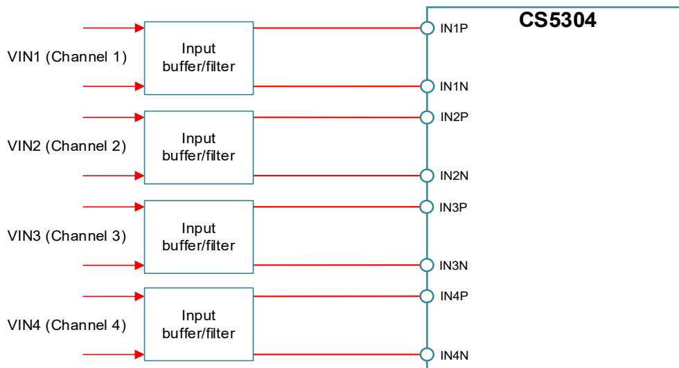
Figure 21: No Output Summing
