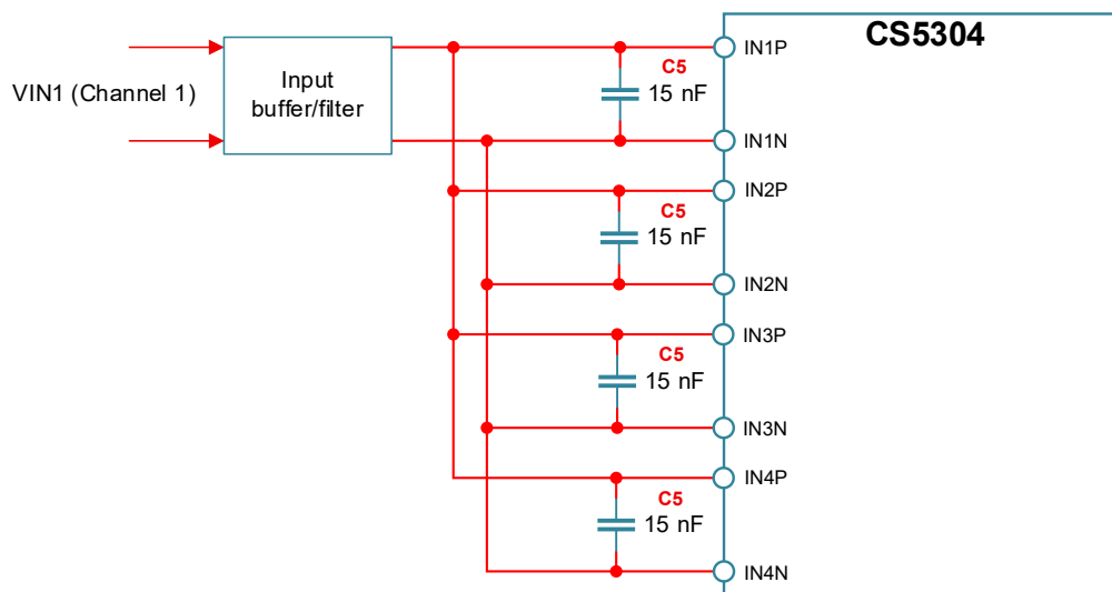
Figure 23: ADC Inputs Combined in a Group of 4
