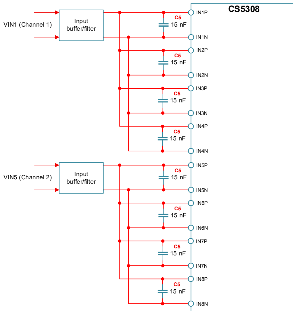
Figure 26: ADC Inputs Combined in Groups of 4
