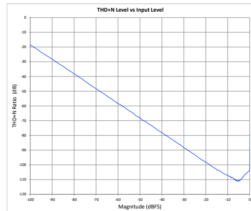
Figure 31: THD+N ratio Vs Magnitude
