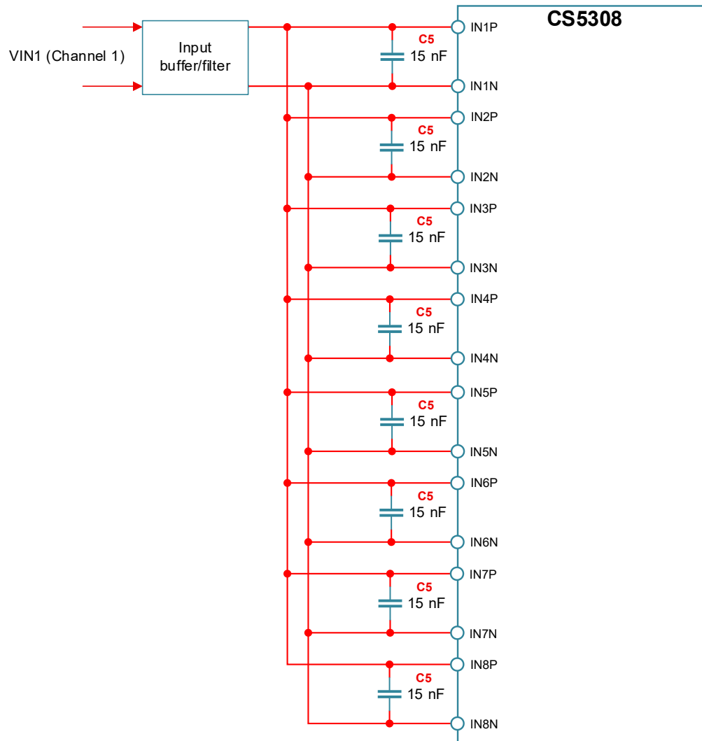
Figure 27: ADC Inputs Combined in a Group of 8
