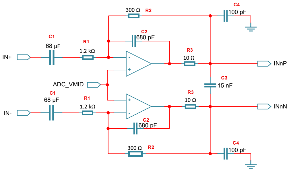
Figure 20: Differential Input Buffer for Input Summing
