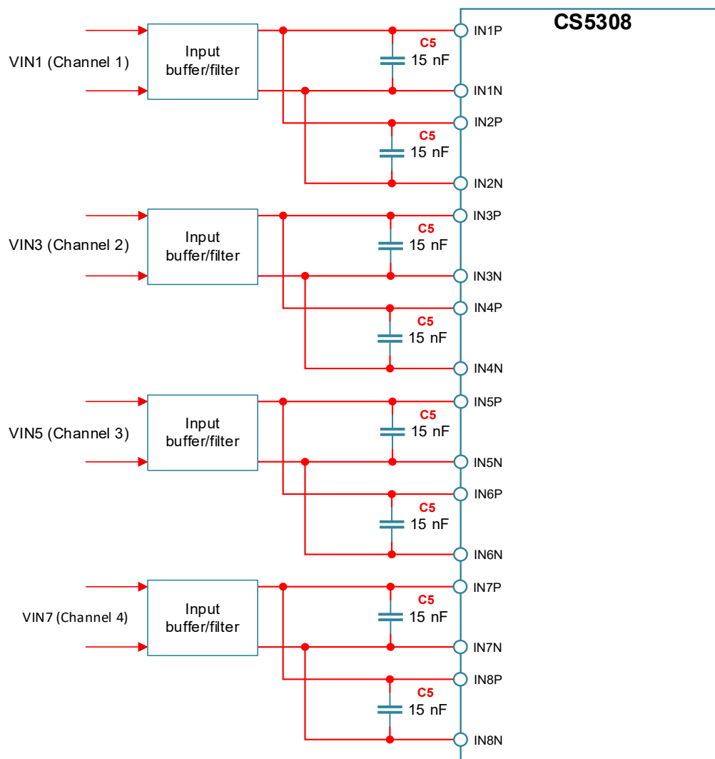
Figure 25: ADC Inputs Combined in Groups of 2
