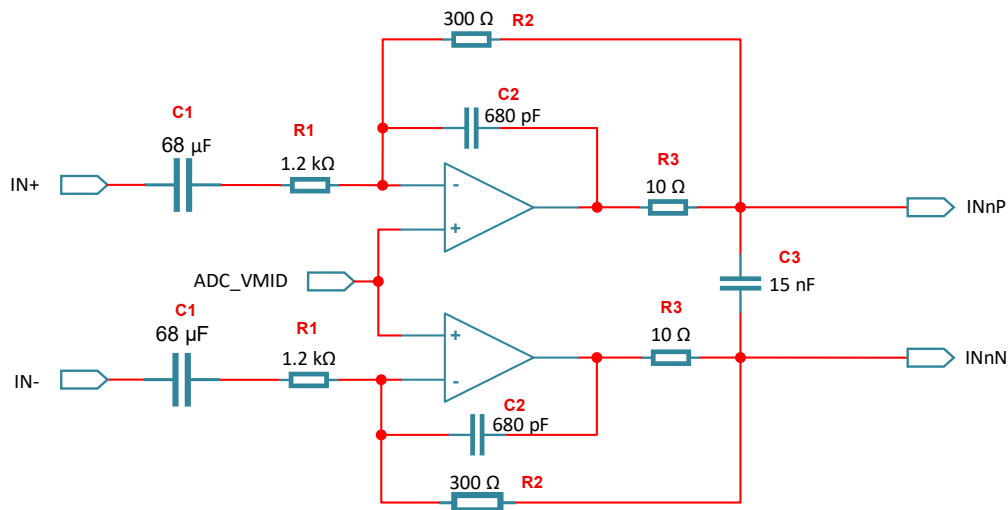
Figure 19: Differential Input Buffer
