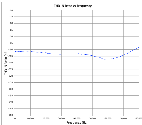
Figure 44: -1dBFS THD+N ratio Vs Frequency
