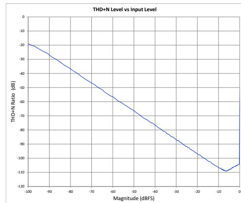
Figure 45: THD+N ratio Vs Magnitude
