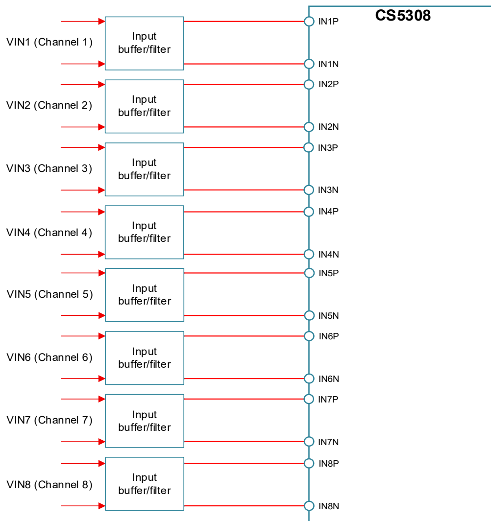
Figure 24: No Output Summing
