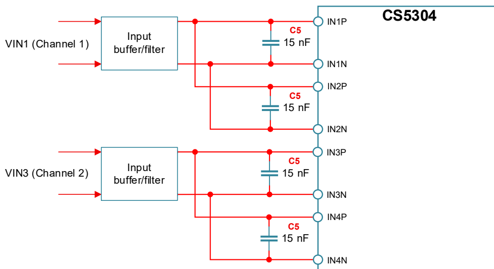
Figure 22: ADC Inputs Combined in Groups of 2
