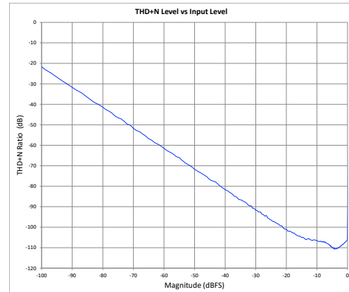
Figure 29: THD+N ratio Vs Magnitude
