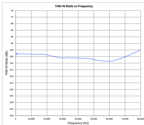
Figure 32: -1dBFS THD+N ratio Vs Frequency
