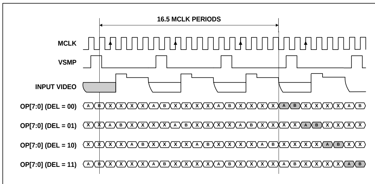
Figure 24 Mode 2 Operation
