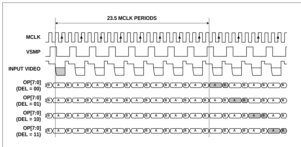
Figure 25 Mode 3 Operation
