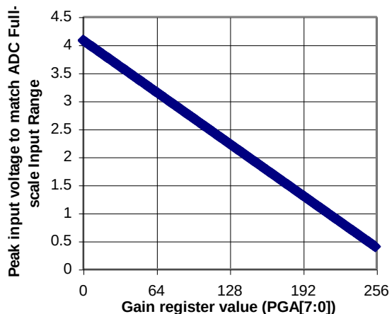
Figure 15 Peak Input Voltage to Match ADC Full-scale Range
