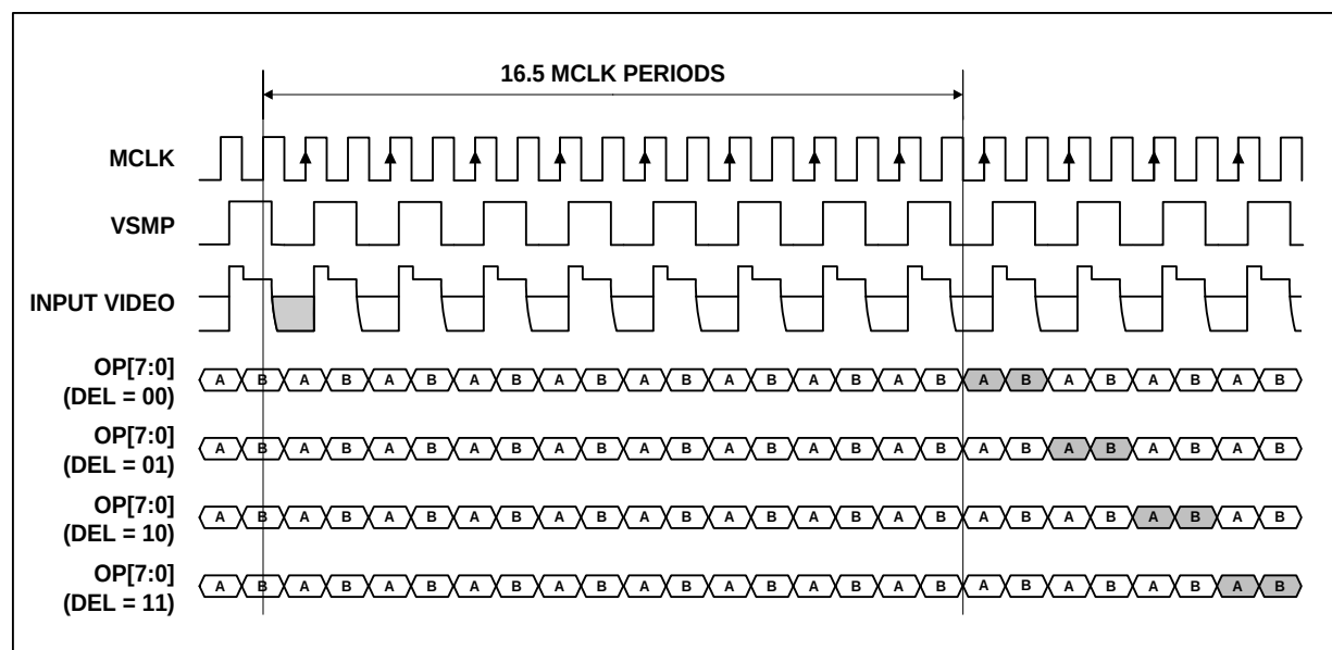
Figure 26 Mode 4 Operation
