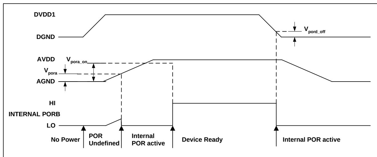
Figure 10 Typical Power up Sequence where DVDD1 is Powered before AVDD
