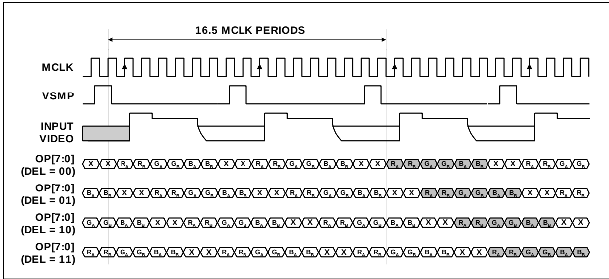
Figure 27 Mode 5 Operation (MCLK:VSMP Ratio = 8:1)
