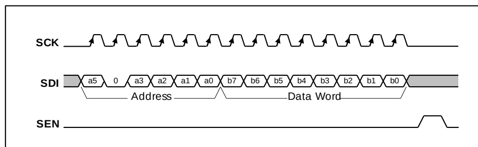
Figure 19 Serial Interface Register Write
