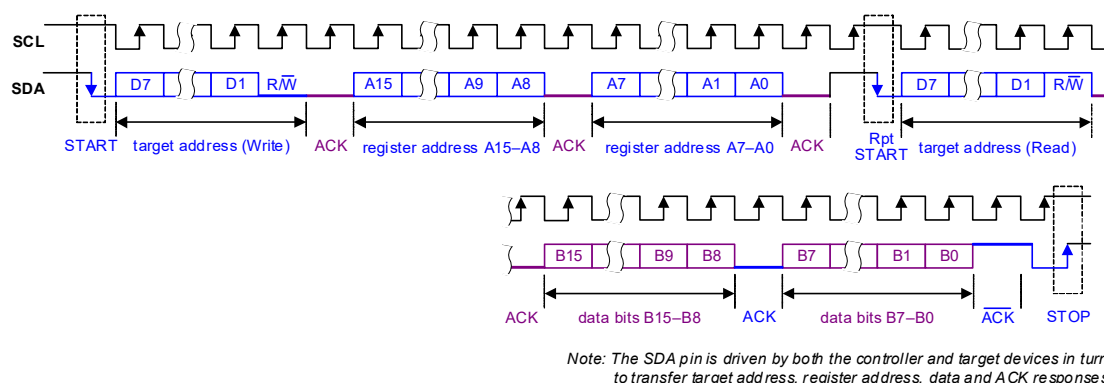
Figure 4-33. Control Interface I 2 C Register Read
