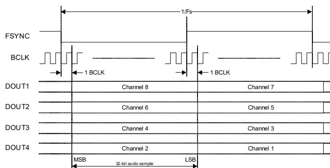
Figure 4-31. Reverse Channel Order
