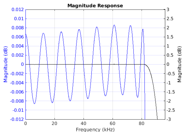
Figure 7-31. Passband Magnitude
