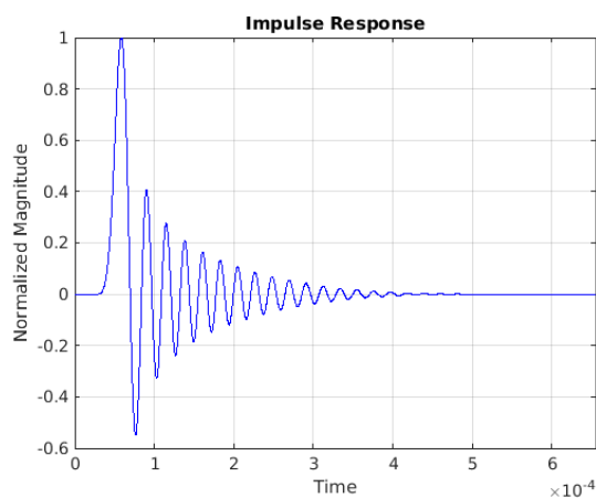
Figure 7-22. Impulse Response—Minimum Phase
