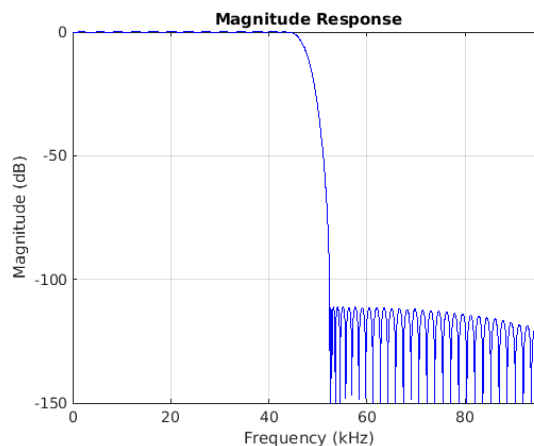
Figure 7-20. Stopband Magnitude
