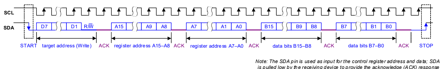
Figure 4-32. Control Interface I 2 C Register Write
