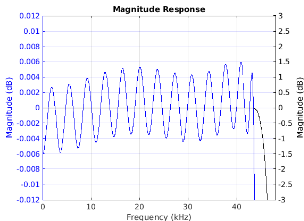
Figure 7-19. Passband Magnitude
