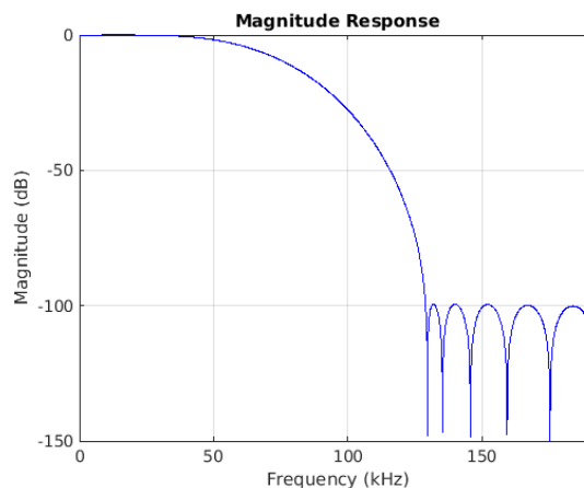
Figure 7-38. Stopband Magnitude
