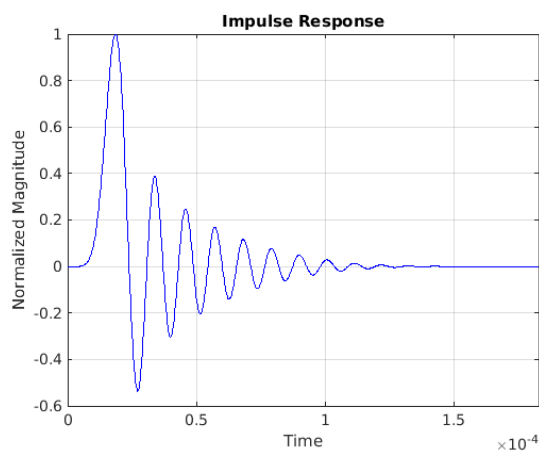
Figure 7-34. Impulse Response—Minimum Phase
