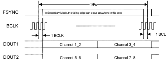
Figure 4-21. TDM Data Format—2 x DOUT
