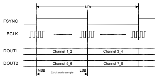
Figure 4-19. Left-Justified Data Format
