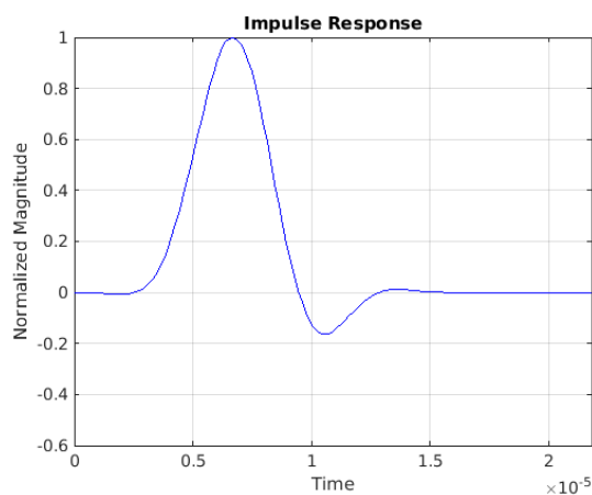
Figure 7-52. Impulse Response—Minimum Phase
