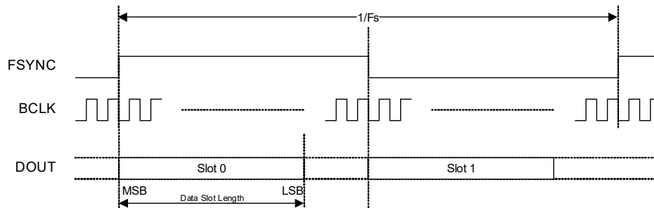
Figure 4-9. Left-Justified Data Format
