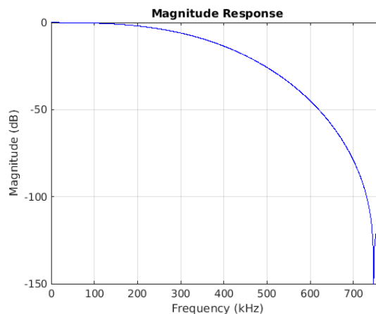
Figure 7-62. Stopband Magnitude
