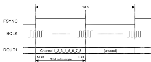
Figure 4-28. Left-Justified Data Format
