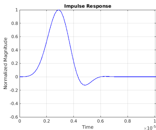
Figure 7-64. Impulse Response—Minimum Phase
