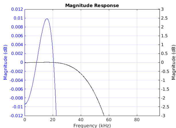
Figure 7-37. Passband Magnitude
