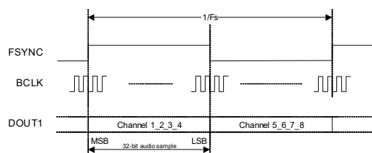
Figure 4-24. Left-Justified Data Format
