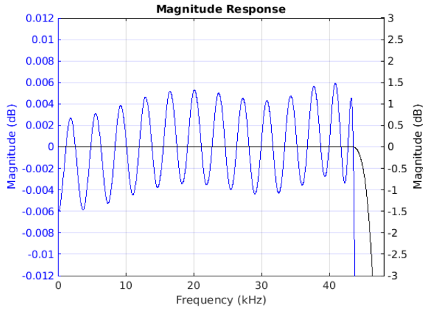
Figure 8-19. Passband Magnitude
