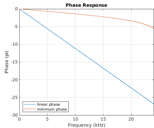
Figure 8-11. Phase vs. Frequency
