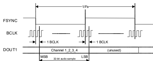
Figure 4-22. I 2 S Data Format
