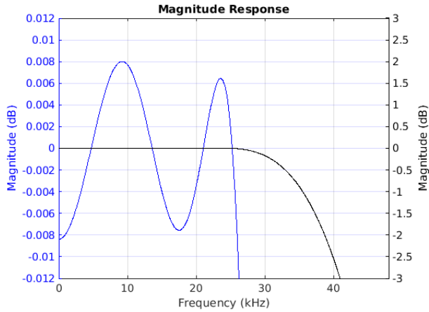
Figure 8-25. Passband Magnitude
