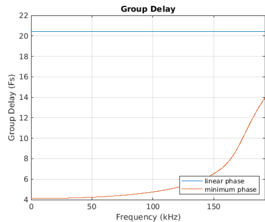
Figure 8-48. Group Delay vs. Frequency
