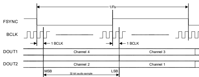
Figure 4-26. Reverse Channel Order
