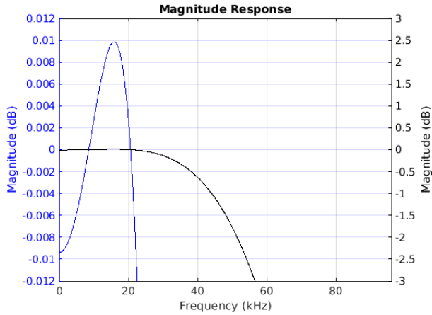
Figure 8-37. Passband Magnitude
