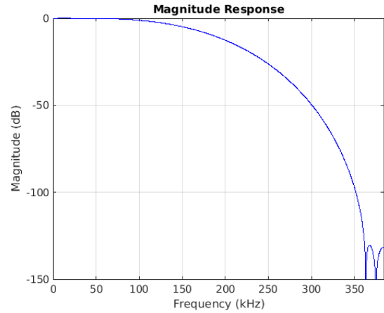
Figure 8-50. Stopband Magnitude
