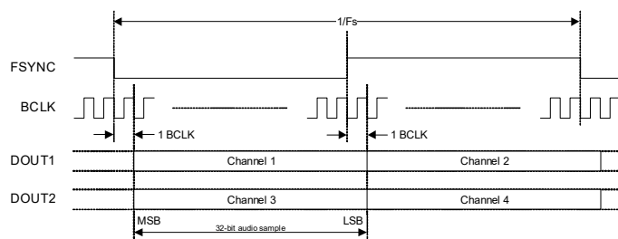
Figure 4-25. Default Channel Order
