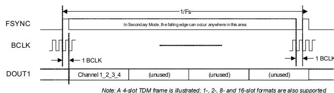
Figure 4-24. TDM Data Format
