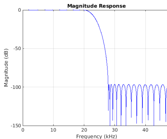
Figure 8-14. Stopband Magnitude
