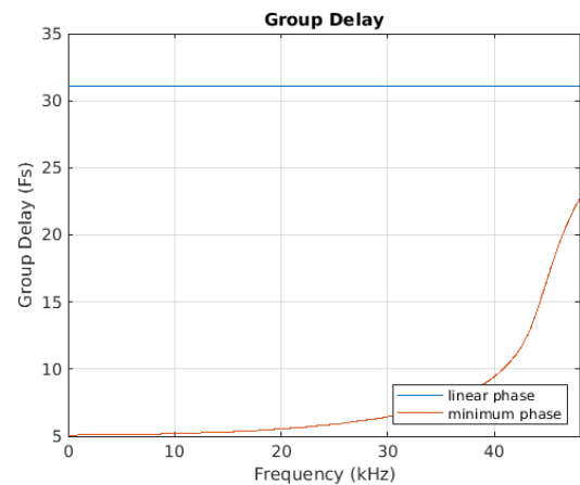
Figure 8-24. Group Delay vs. Frequency
