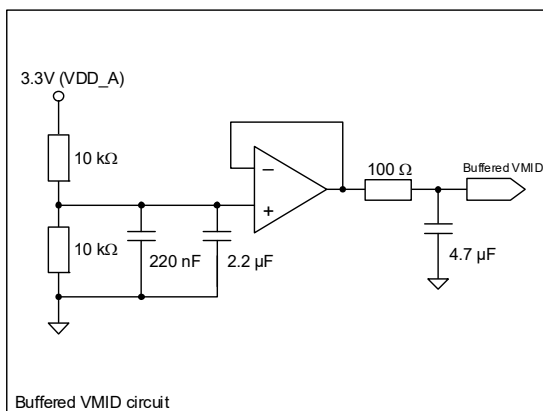
Figure 2-2. Typical Connections—Using External VMID Reference
