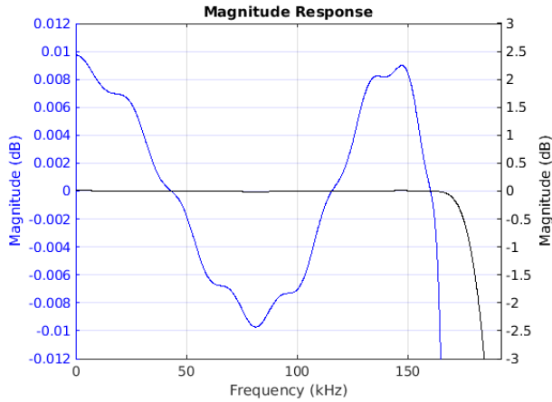
Figure 8-43. Passband Magnitude
