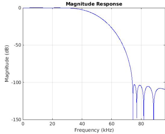
Figure 8-26. Stopband Magnitude
