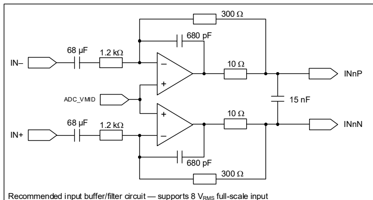
Figure 2-1. Typical Connections—Using Internal VMID Reference
