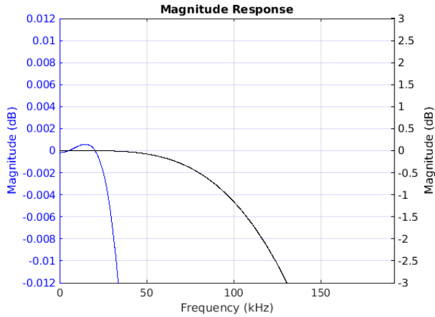
Figure 8-49. Passband Magnitude
