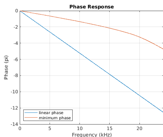
Figure 8-17. Phase vs. Frequency
