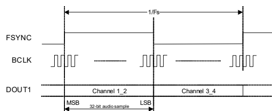
Figure 4-19. Left-Justified Data Format
