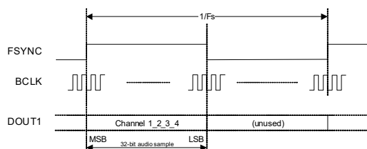
Figure 4-23. Left-Justified Data Format
