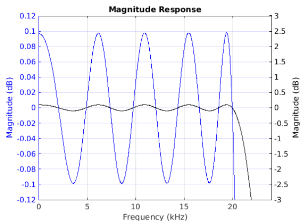
Figure 8-13. Passband Magnitude
