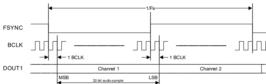
Figure 4-12. I 2 S Data Format
