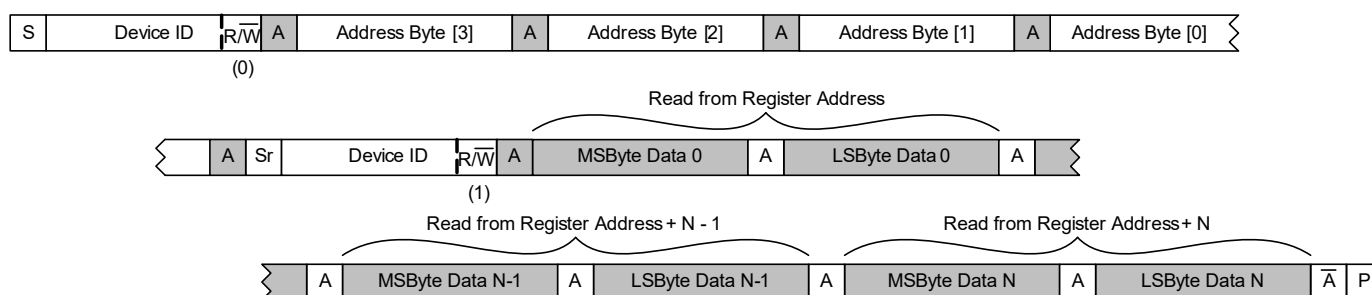
Figure 4-74. Multiple-Register Read from Specified Address
