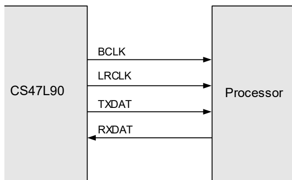
Figure 4-37. Master Mode
