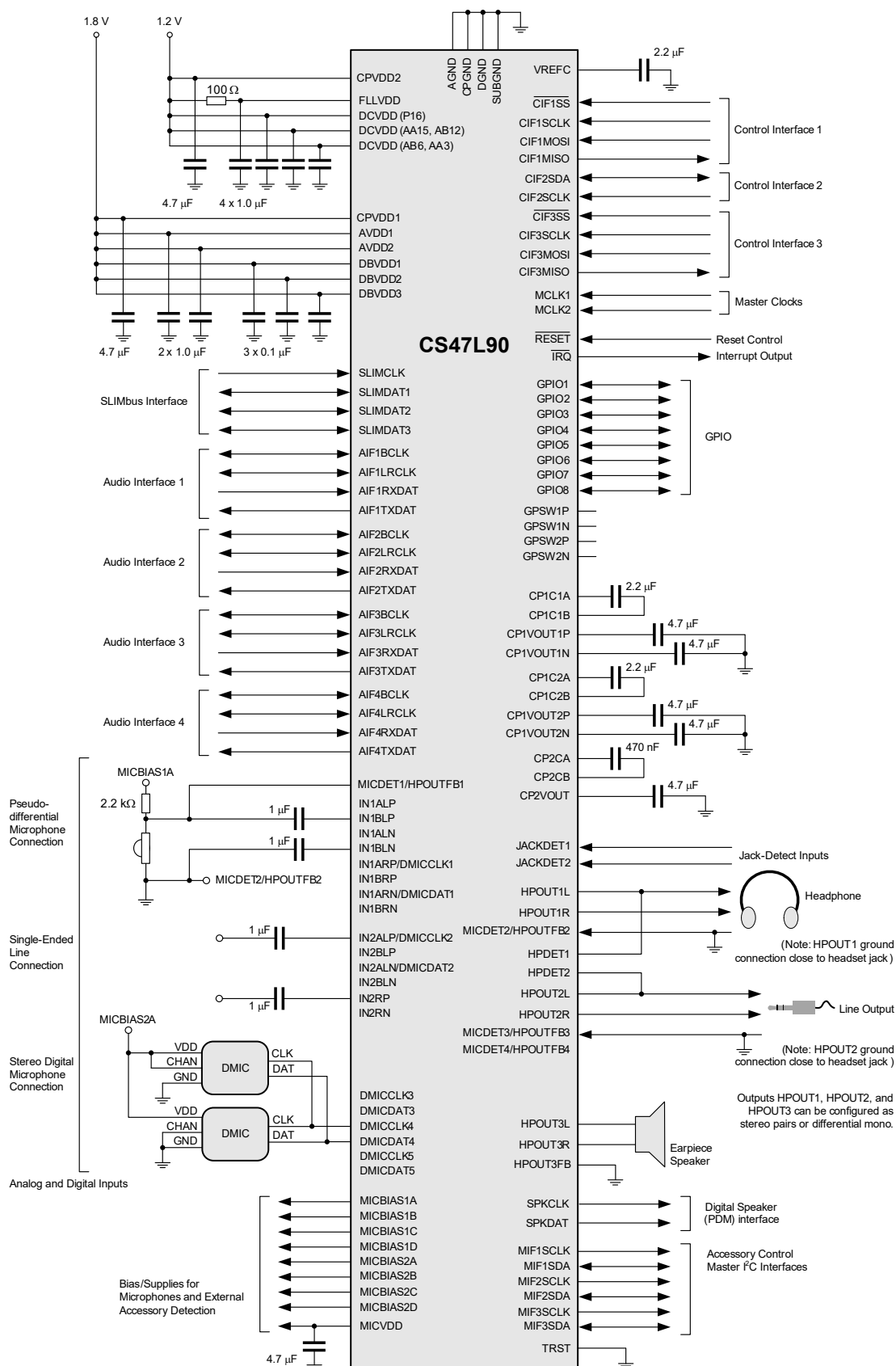
Figure 2-1. Typical Connection Diagram
