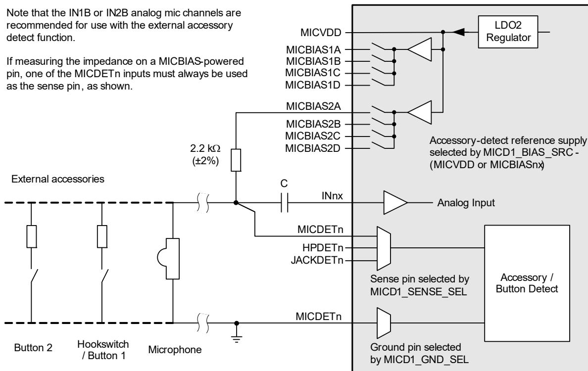
Figure 4-59. Microphone- and Accessory-Detect Interface
