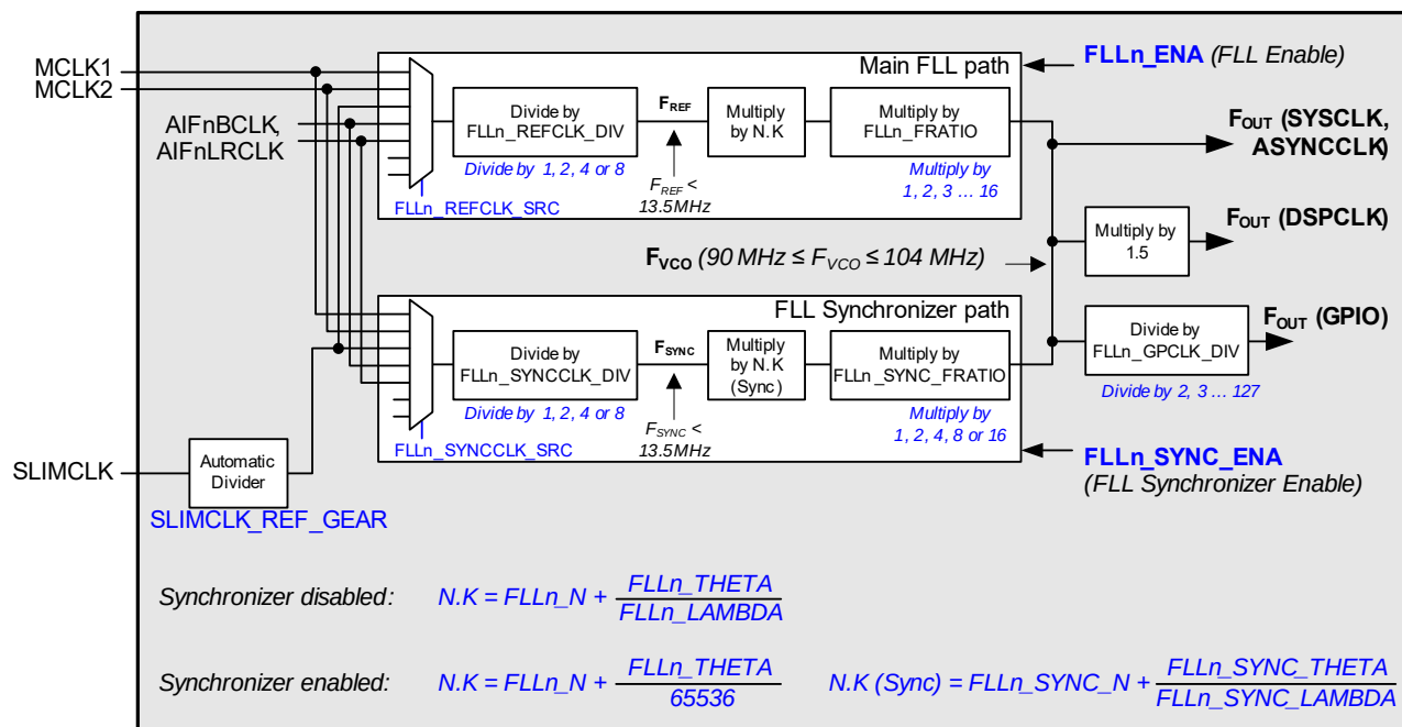
Figure 4-65. FLL1/FLL2 Configuration
