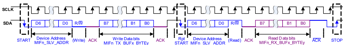
Figure 4-33. Master I 2 C Write and Read
