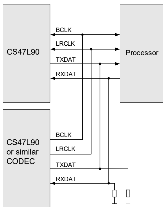
Figure 4-48. TDM with Other Codec as Master
