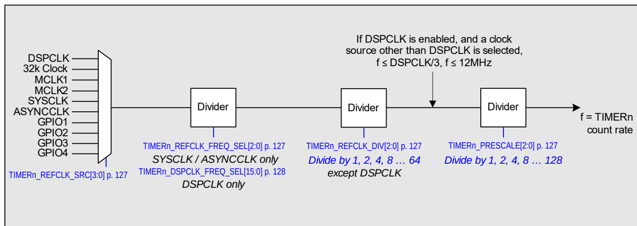
Figure 4-34. General-Purpose Timer
