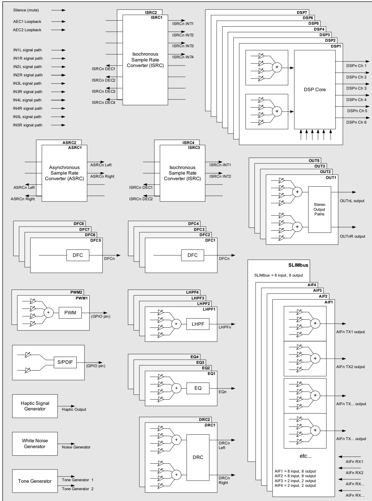
Figure 4-11. Digital Core
