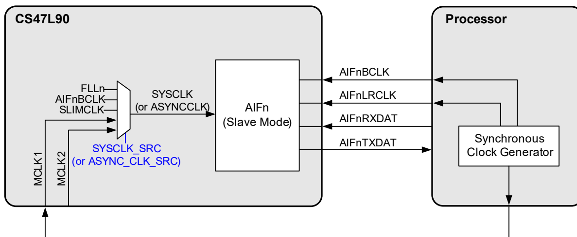
Figure 5-13. AIF Slave Mode, Using MCLK as Reference
