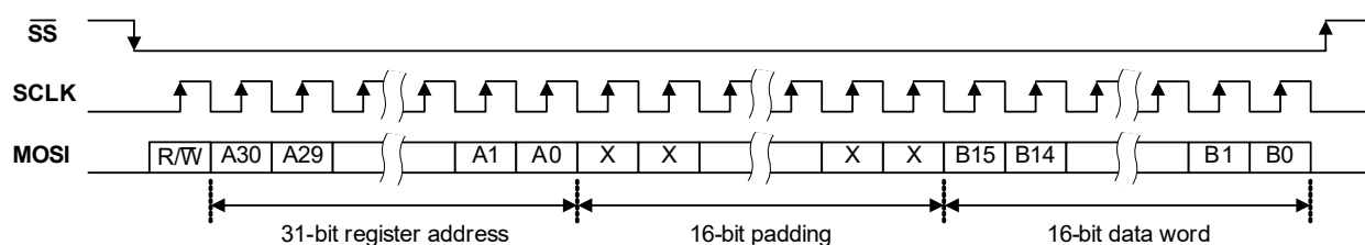
Figure 4-67. Control Interface SPI Register Write (16-Bit Data Words)
