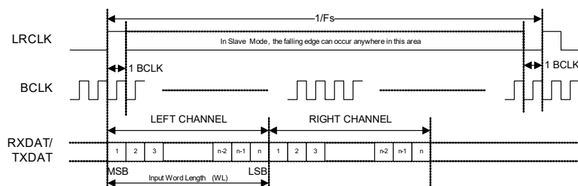
Figure 4-40. DSP Mode B Data Format
