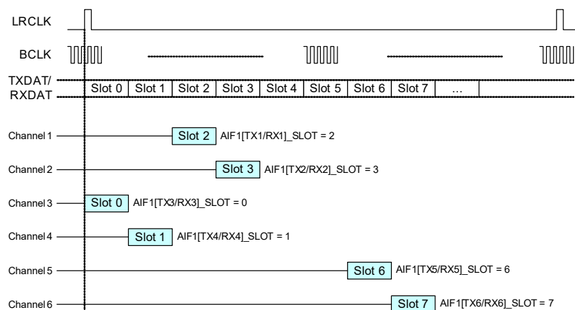
Figure 4-44. DSP Mode B Example
