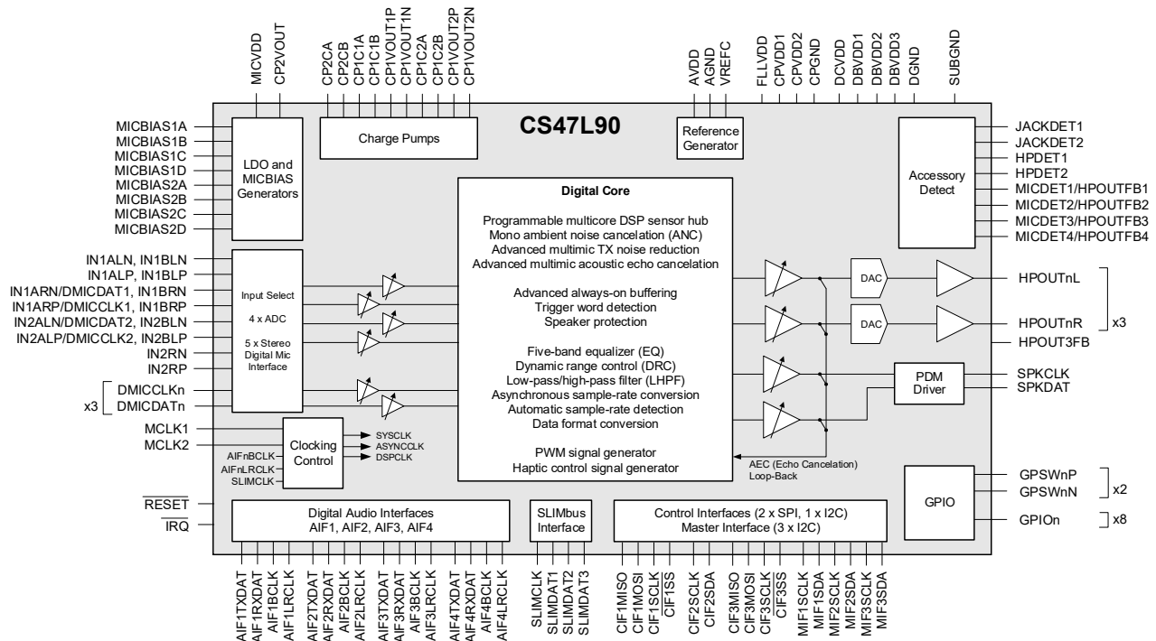
Figure 4-1. CS47L90 Block Diagram
