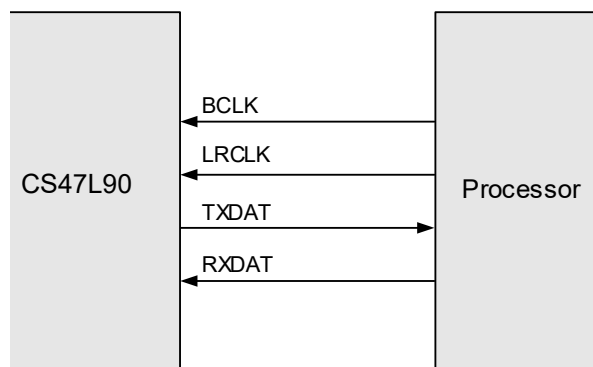
Figure 4-38. Slave Mode
