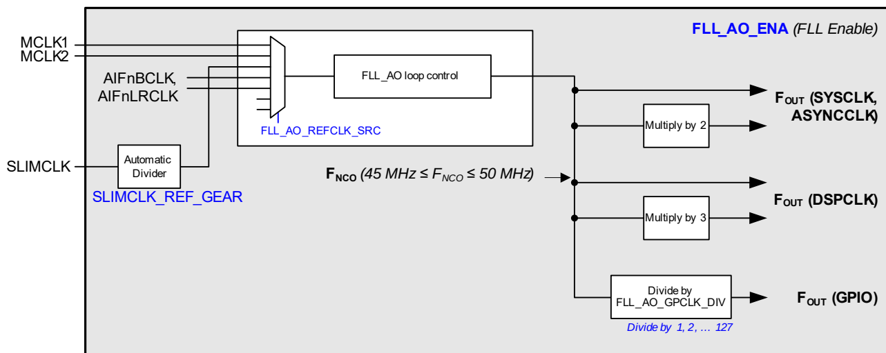
Figure 4-66. FLL_AO Configuration
