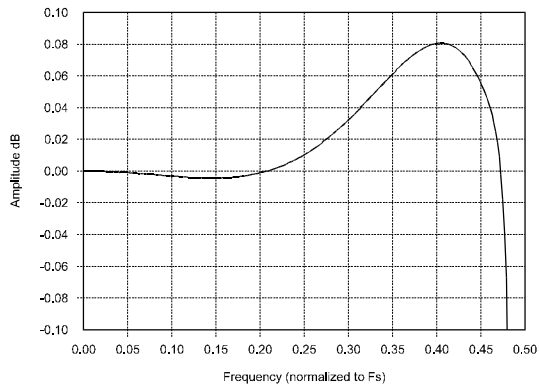
Figure 27. Passband Ripple
