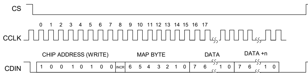
Figure 18. Control Port Timing in SPI Mode
