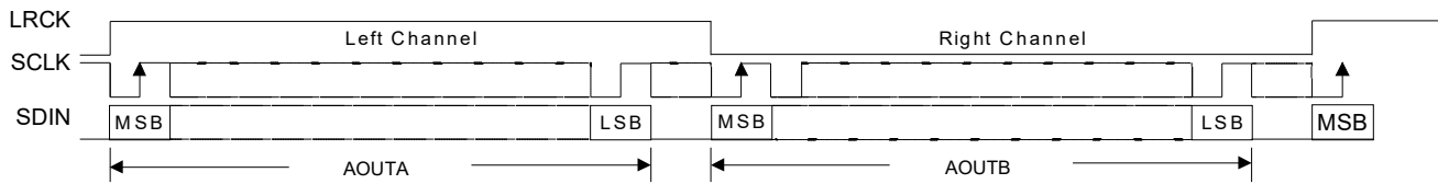
Figure 15. Left-Justified Format
