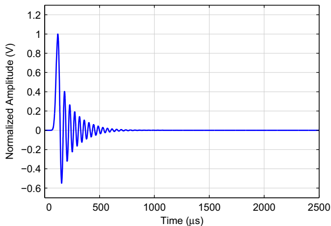
Figure 9-16. Impulse Response—Minimum Phase
