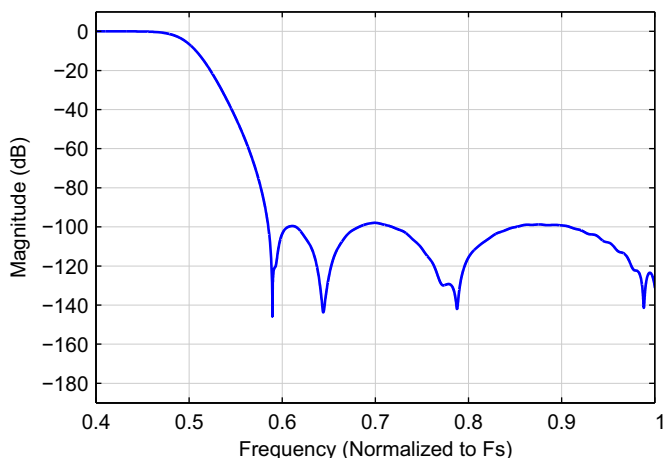
Figure 9-14. Stopband Attenuation
