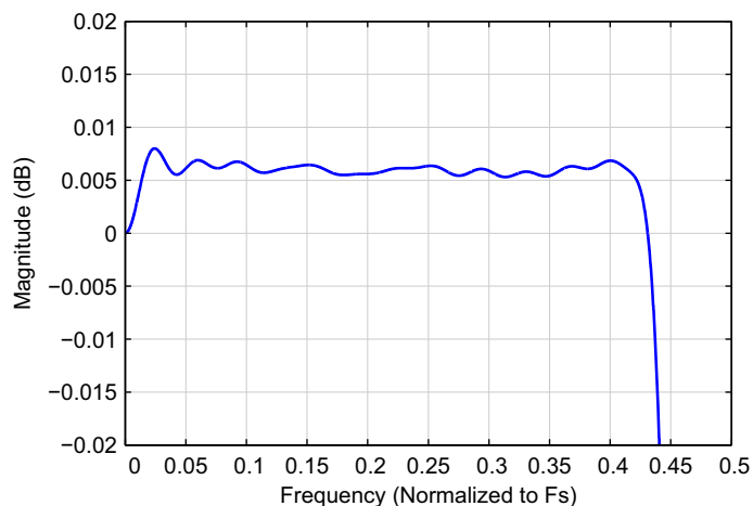
Figure 9-13. Passband Ripple
