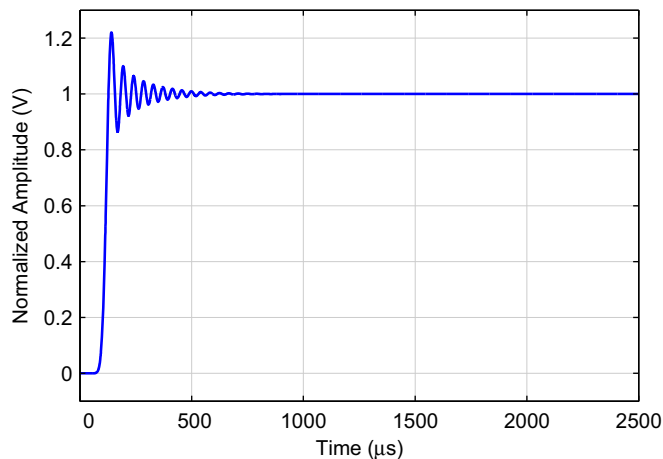
Figure 9-18. Step Response—Minimum Phase
