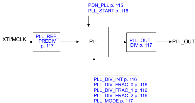
Figure 4-18. Fractional-N PLL
