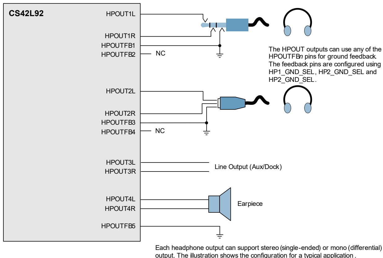
Figure 4-54. Headphone and Earpiece Connection
