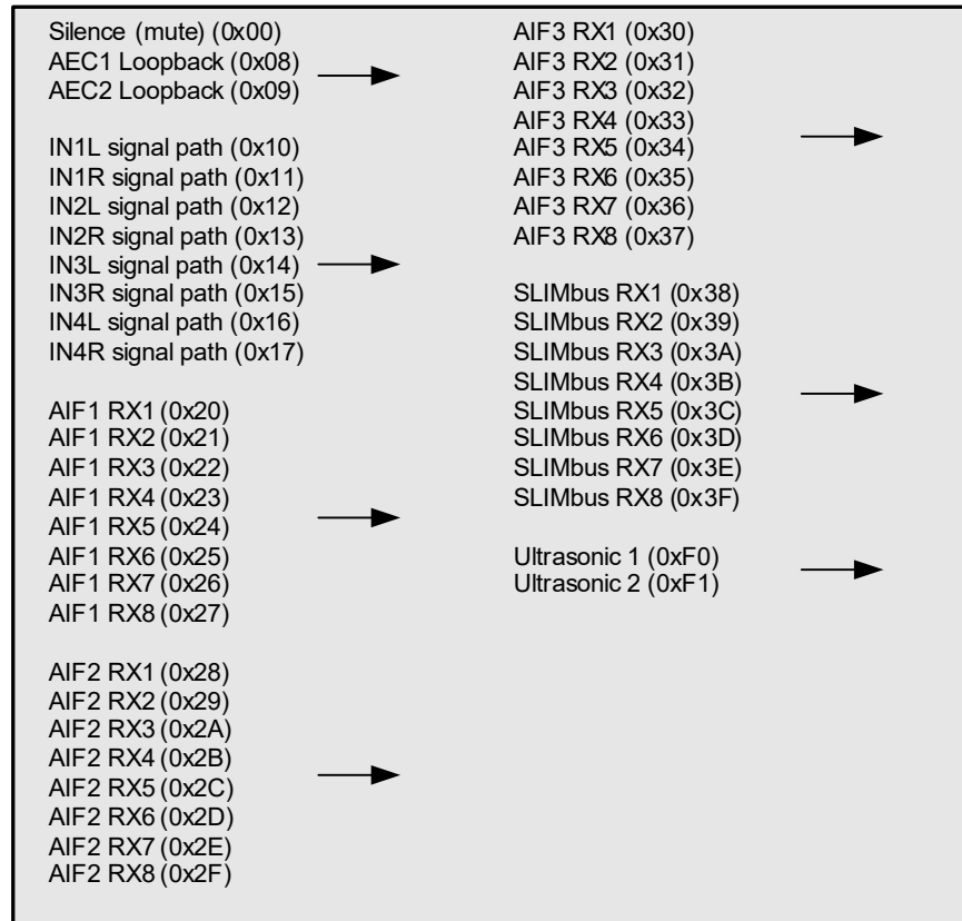
Figure 4-16. Digital-Core Inputs
