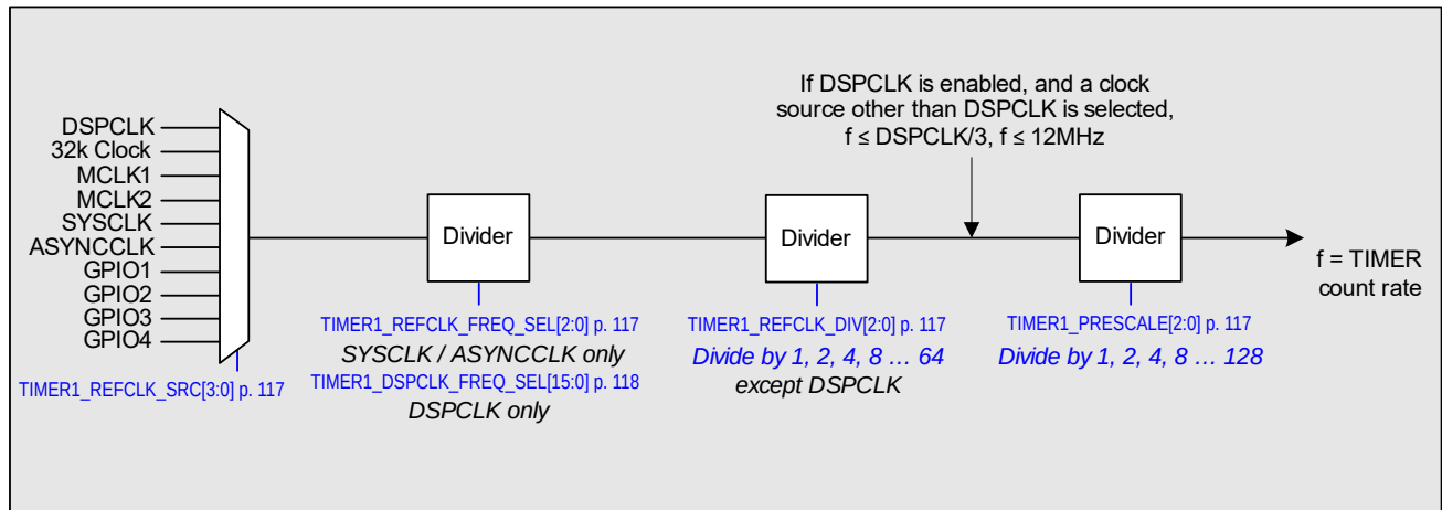
Figure 4-35. General-Purpose Timer
